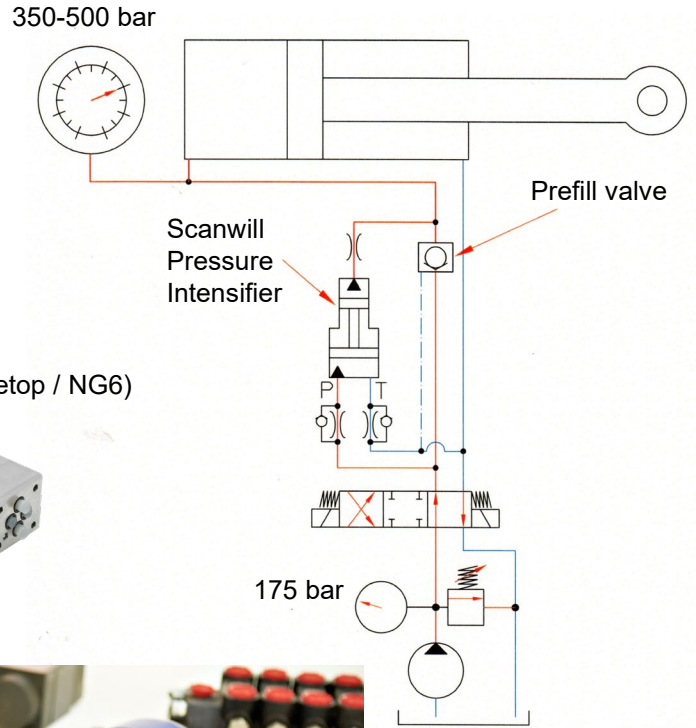
The MP-M intensifier (in-line)
